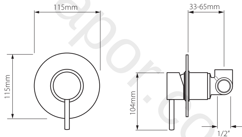
zoo concealed single lever shower valve with round backplate
