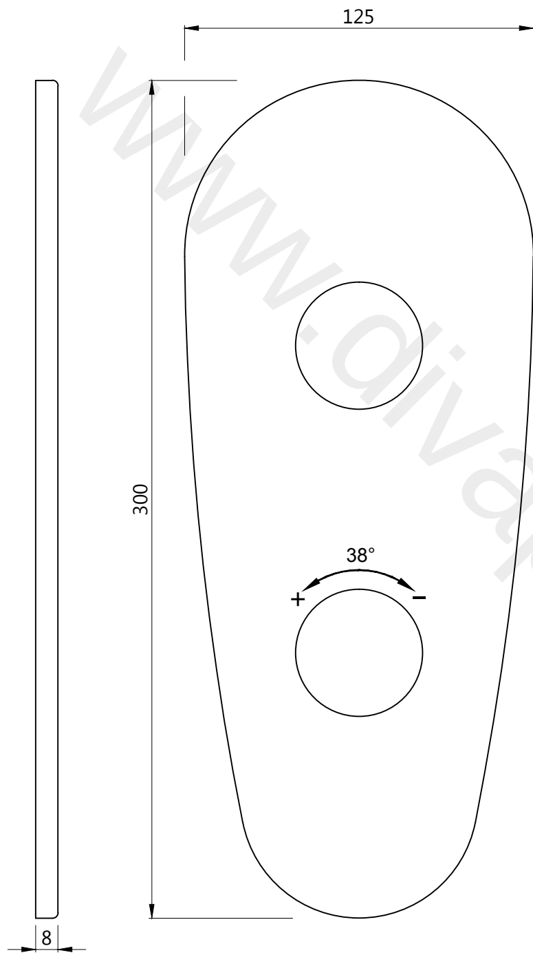
WALL FLANGE
