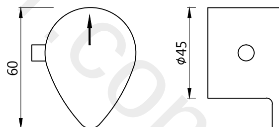
THERMOSTATE HANDLE
