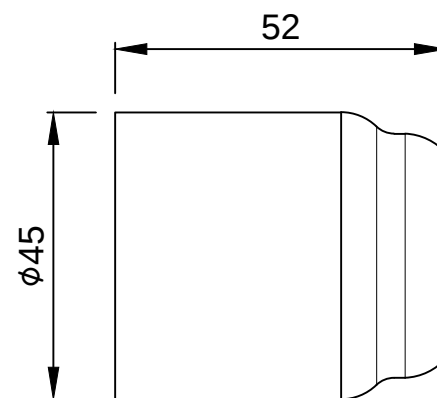
CARTRIDGE SLEEVE
