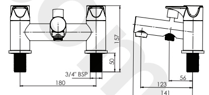
Bath Shower Mixer UNDEBSM
