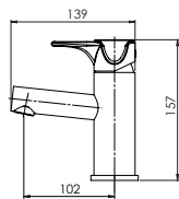
Basin Mono Mixer Tap* UNDETPBAM
