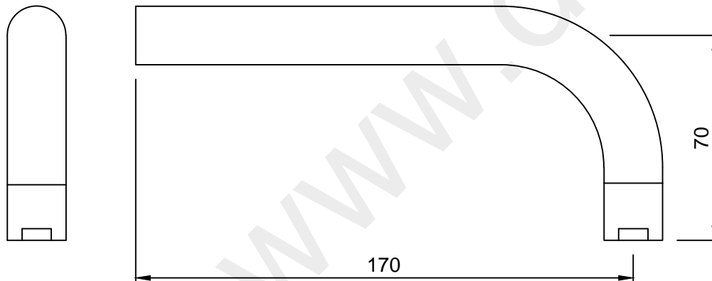
SPOUT
