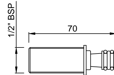
SPOUT NIPPLE
