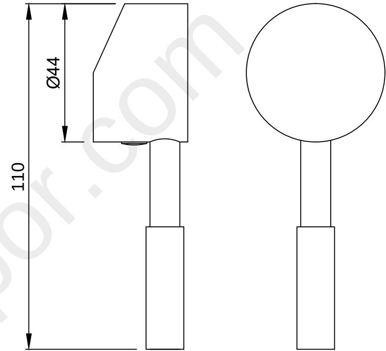
OPERATING LEVER
