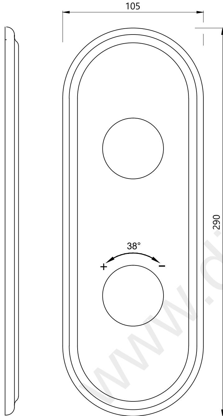
WALL FLANGE
