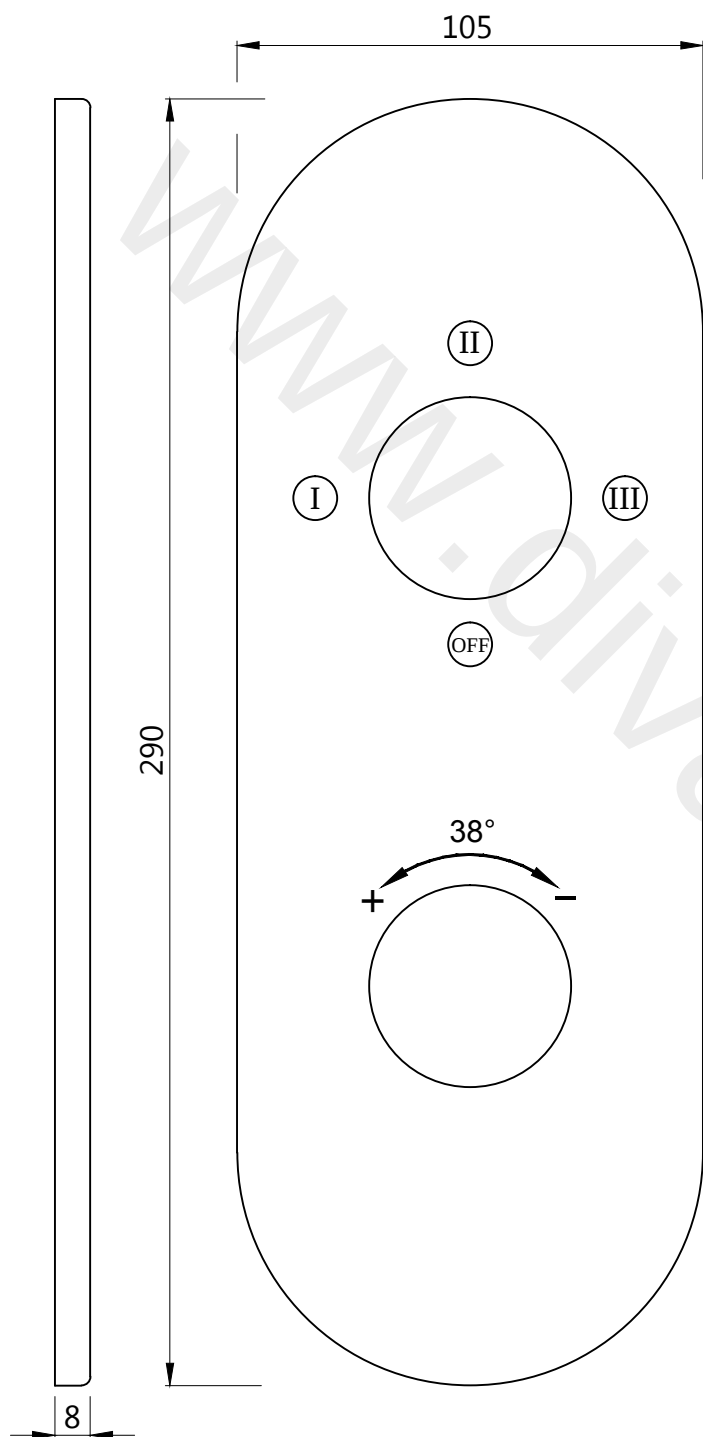
WALL FLANGE
