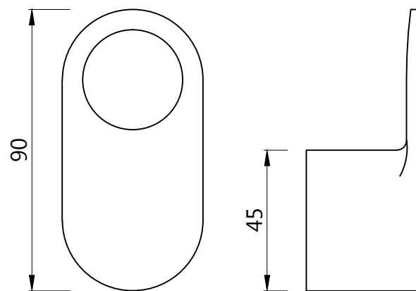
DIVERTER HANDLE
