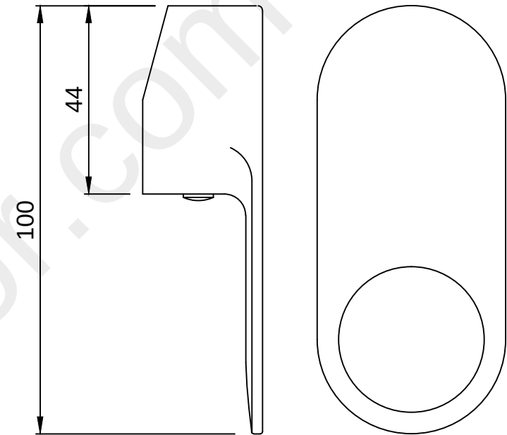
OPERATING LEVER
