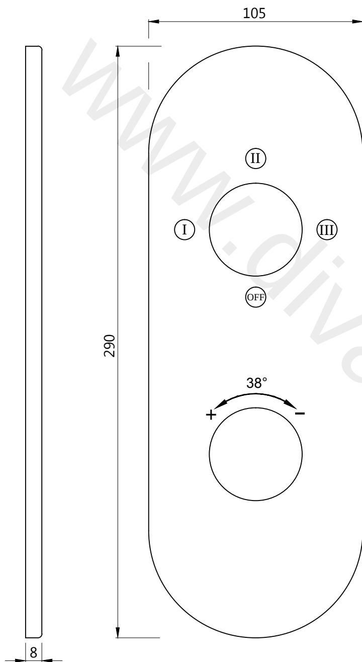
WALL FLANGE
