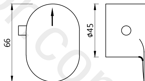
THERMOSTATE HANDLE
