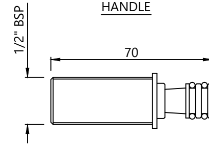
SPOUT NIPPLE
