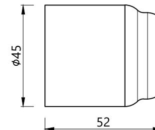
SLEEVE
