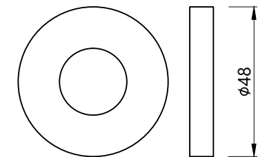
SPOUT SPACER
