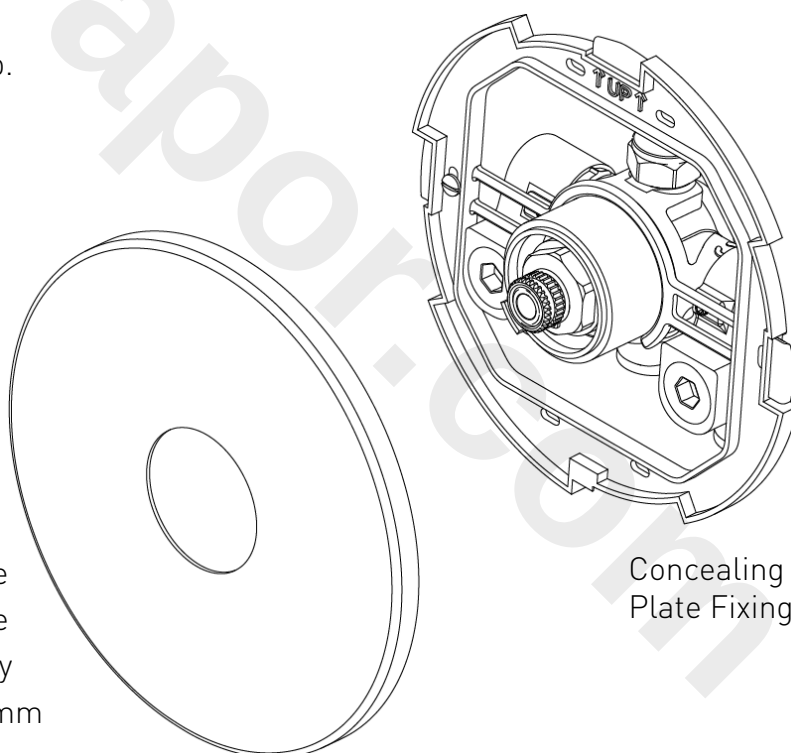
Concealing Plate
