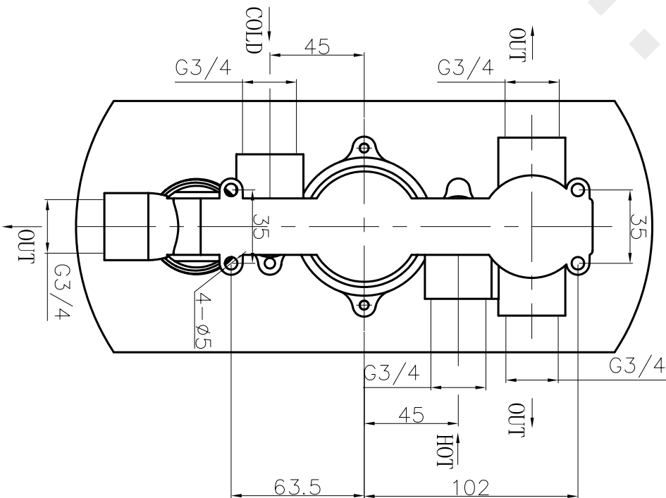
MO3000RC - MODEST THERMOSTATIC SHOWER VALVE 3 Way Portrait
