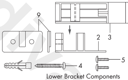
Lower Bracket Components
