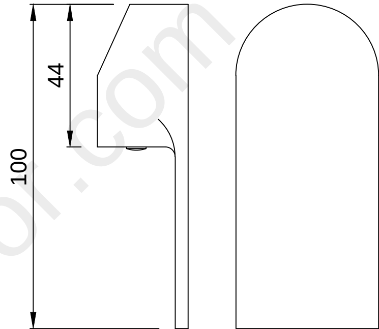
OPERATING LEVER
