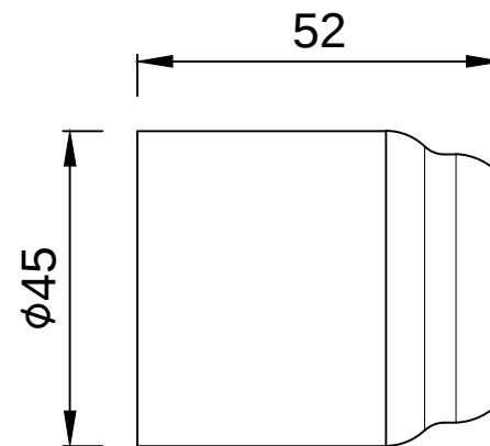
CARTRIDGE SLEEVE
