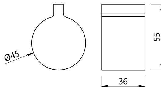
DIVERTER HANDLE
