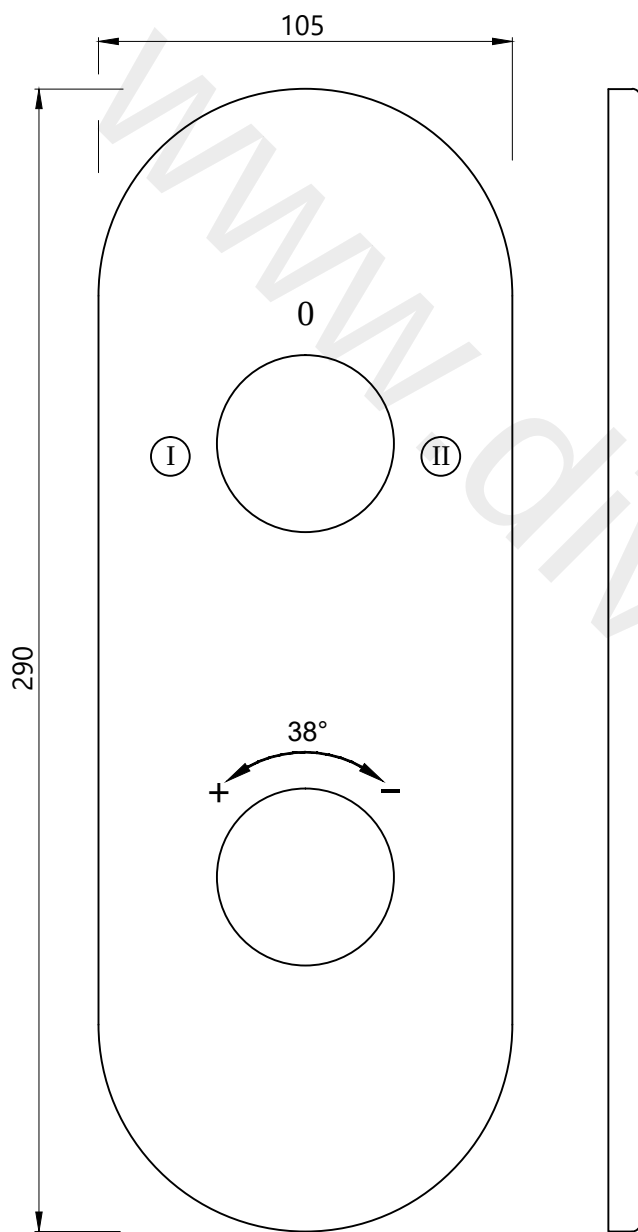
WALL FLANGE
