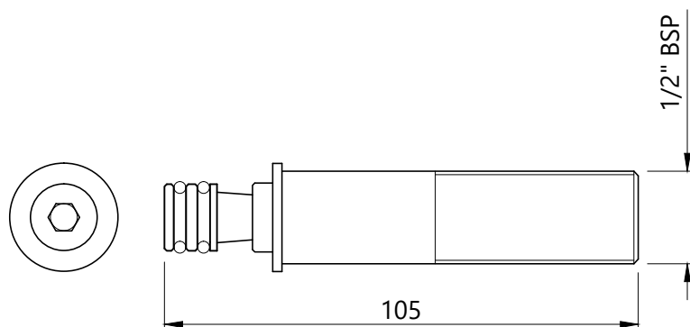
Spout nipple
