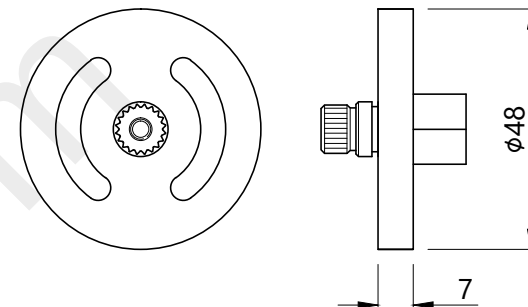
Handle base
