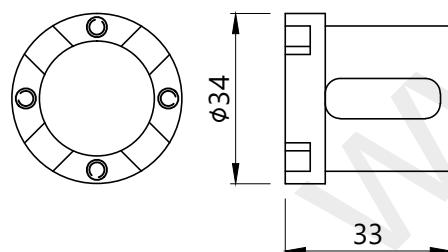
Slotted bush for cartridge
