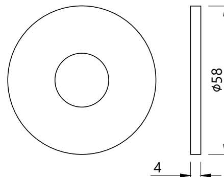
Wall flange
