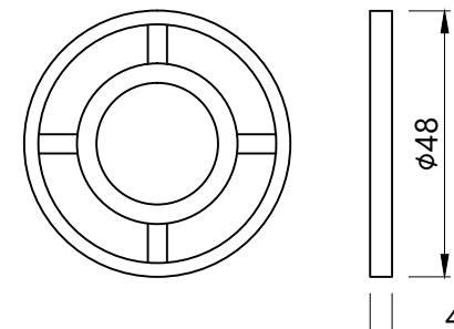
Spout spacer
