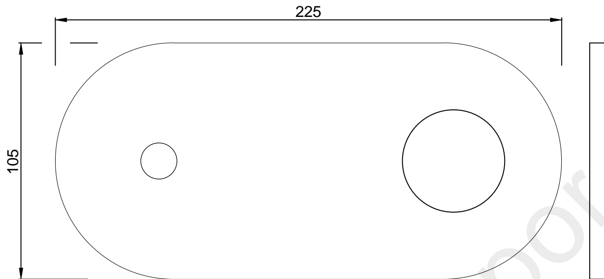
WALL FLANGE
