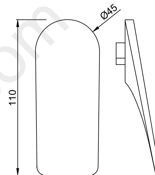
HANDLE
