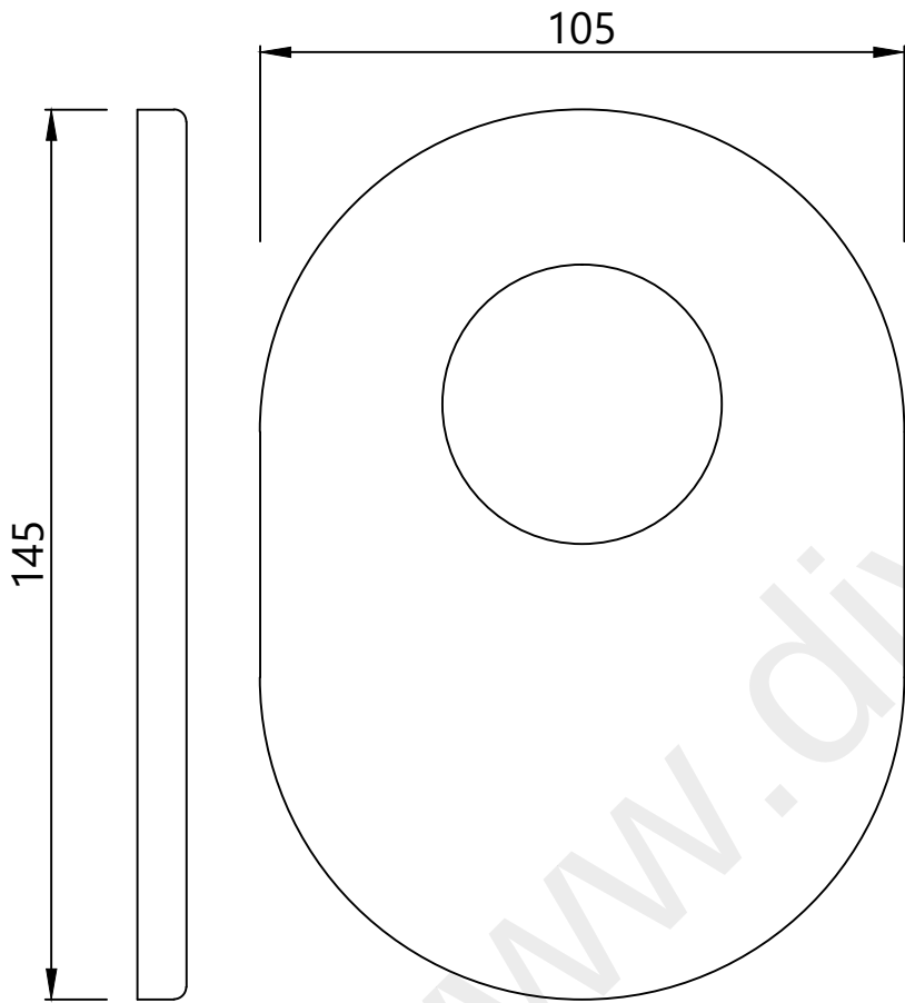
WALL FLANGE
