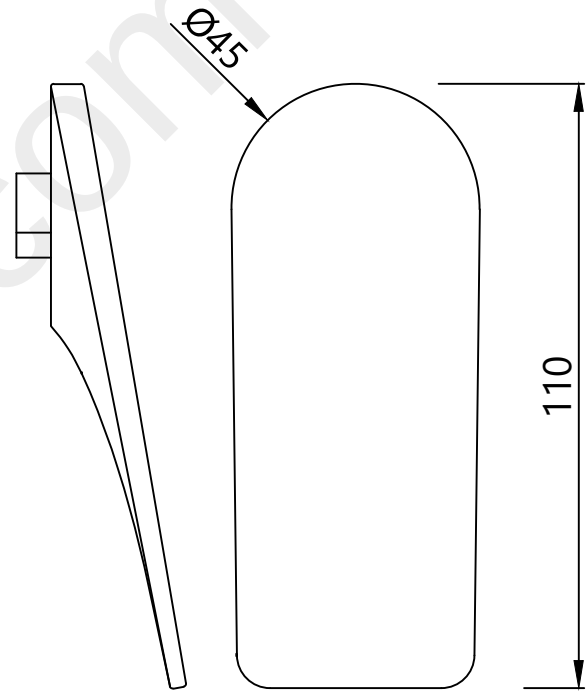
HANDLE
