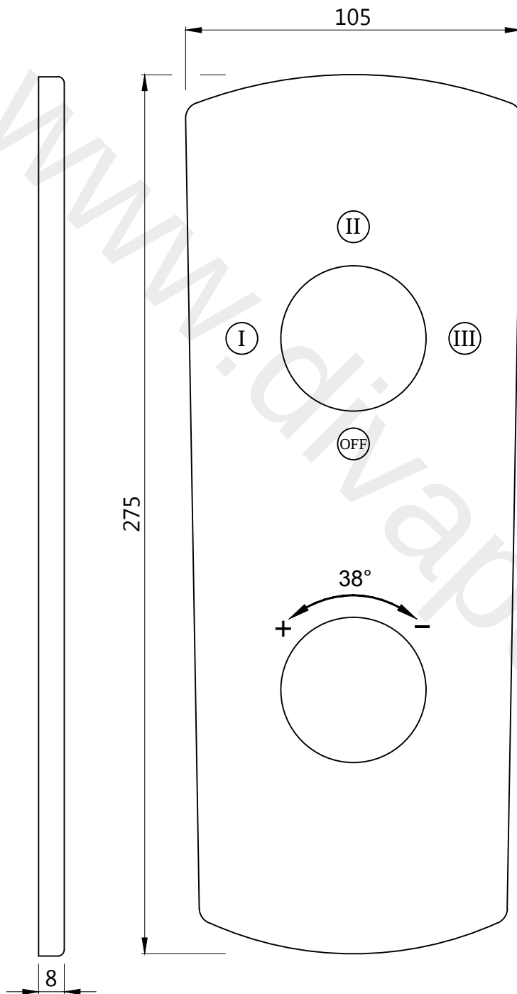
WALL FLANGE
