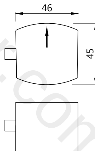
THERMOSTATE HANDLE
