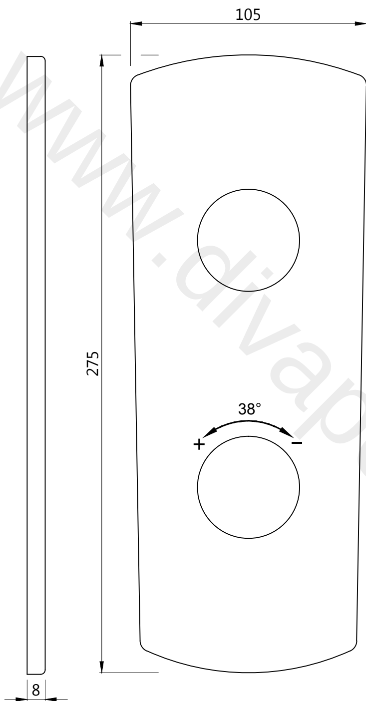
WALL FLANGE
