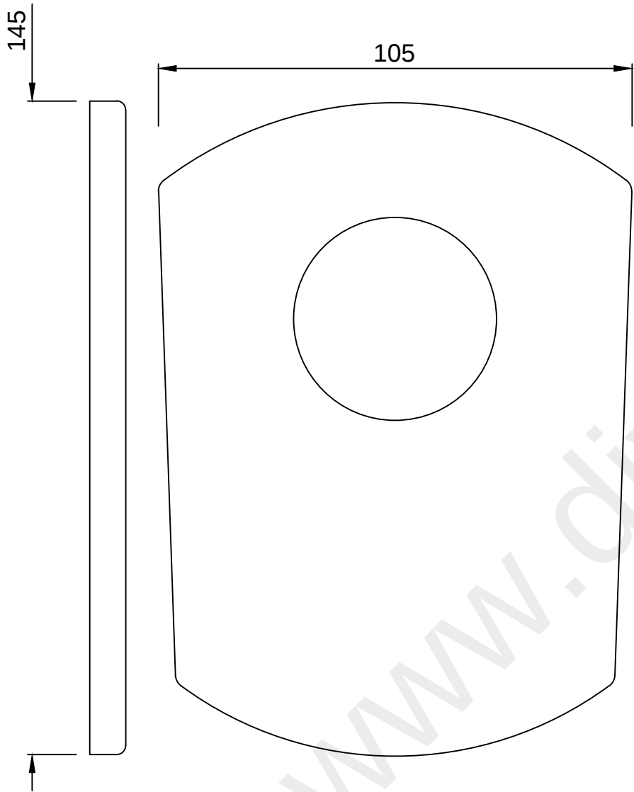
WALL FLANGE
