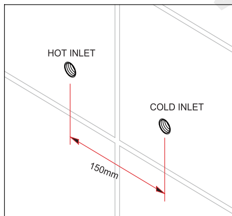
FIG. 1 PREPARING INLET CONNECTIONS
