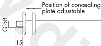
Wall elbow part of EN70001CP rinse station
