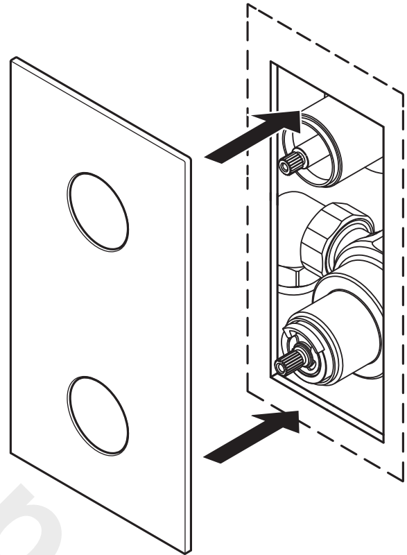
Concealing plate
