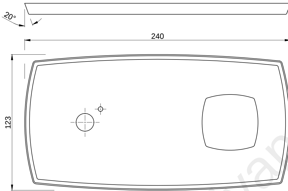
WALL FLANGE
