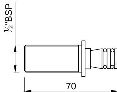
SPOUT NIPPLE
