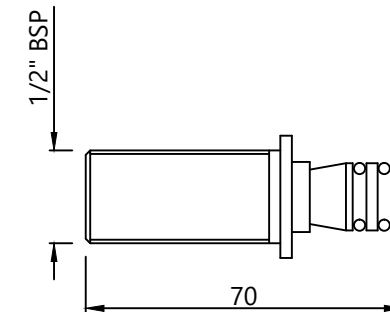
SPOUT NIPPLE
