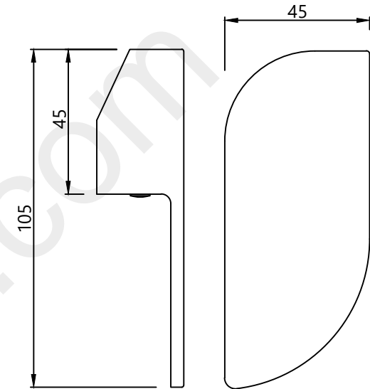
HANDLE
