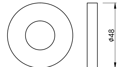
SPOUT SPACER
