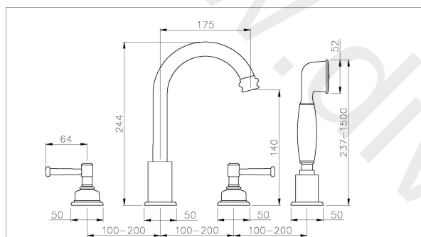
Gallant deck mounted 4 TH bath shower mixer
