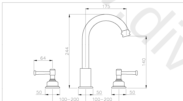
Gallant deck mounted 3 TH bath filler
