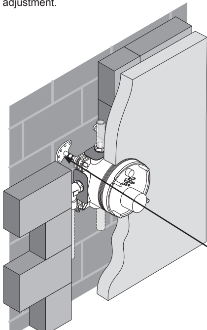
Mounting option C illustrated here using OPTIONAL adjustable fixing legs.
