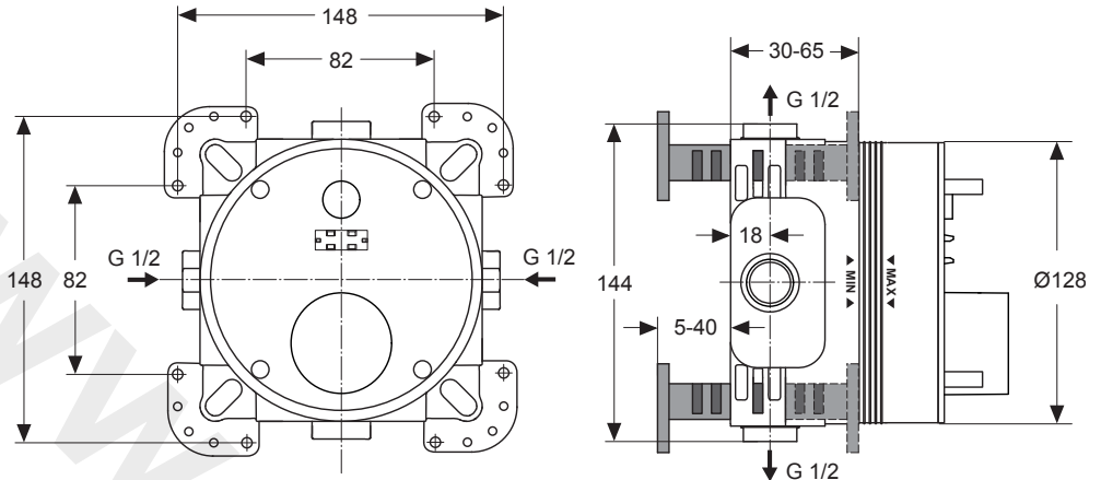
Valve-box dimensions with OPTIONAL legs fitted
