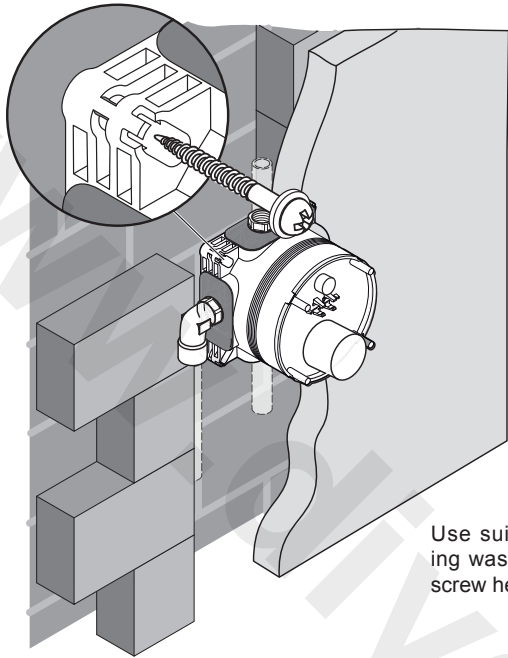
Mounting option A (direct) through the valve-box using the 4 corner slots
