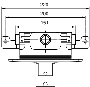
A6456AA square escutcheon shower valve. shown with valve-box, trim & mounting bracket
