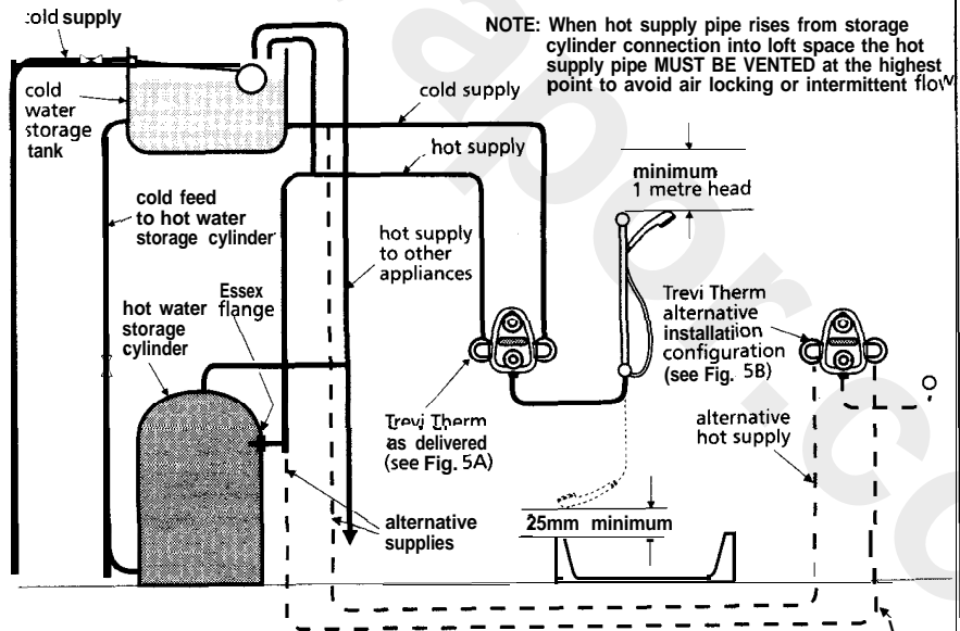
Fig. 3 - for gravity application - showing alternative installation configurations and alternative storage cylinder connections
