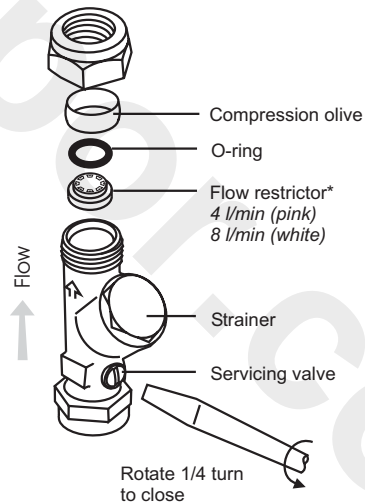
Figure 2 In-line filter and service valve showing restrictor
