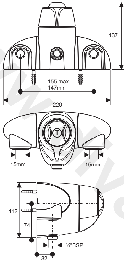
Figure 7 A3101 - Exposed CTV
