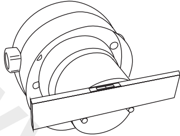
Figure 9 Using spirit level on plaster guard to ensure valve body is level when installing in chased out cavity in a solid wall.
