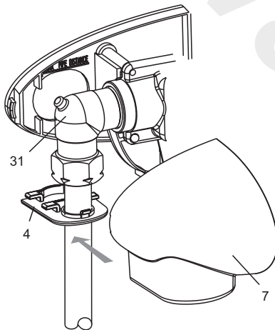
Figure 11 Fitting the cover slips
