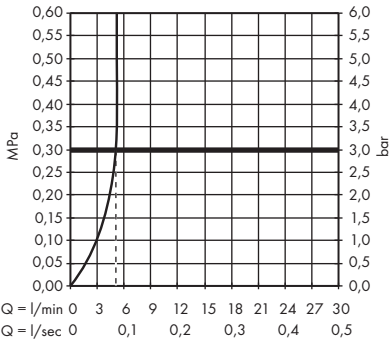
Talis Select S 100 72202000
