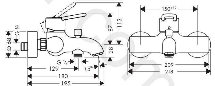
Metropol Puro 33144007
