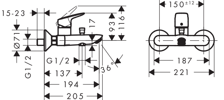
Logis 71400XX7
