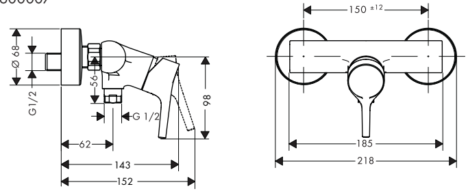
Talis S 72600007
