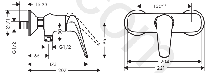
Logis 71600007
