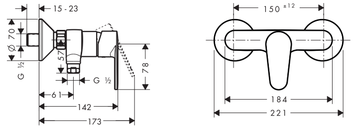
Focus E 31760007
