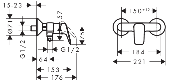
Logis 71600007
