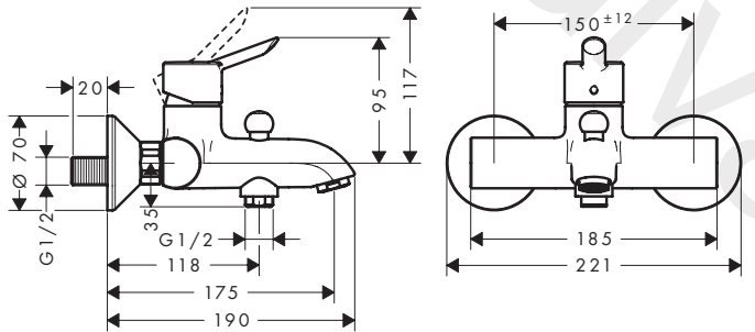
Focus S 31742007
