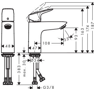
Logis 70 71076000
