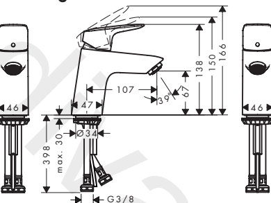
Logis 70 71076000
