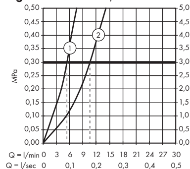
Logis 100 71105000 / 71106000
