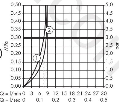
Logis 100 71205000
