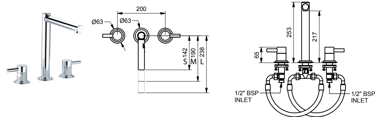
6660 - 6680 Tall Height Deck Mounted Basin Mixer
