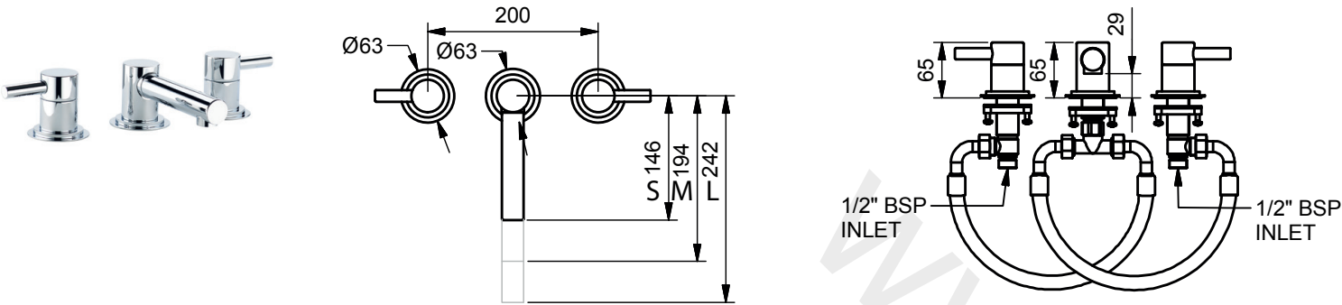
6600 - 6620 Standard Height Deck Mounted Basin Mixer
