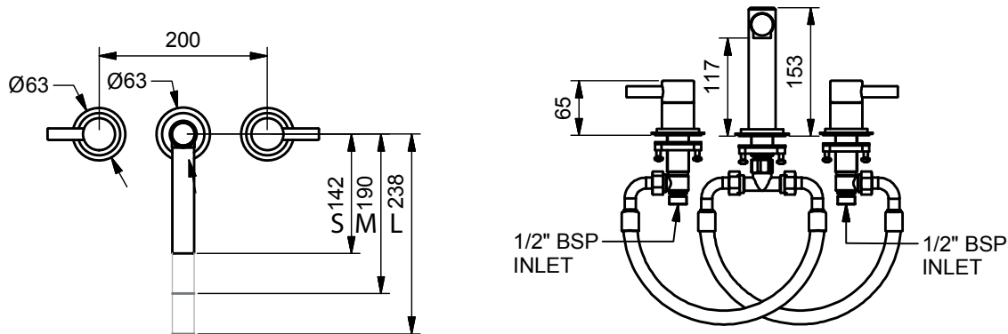
6630 - 6650 Medium Height Deck Mounted Basin Mixer
