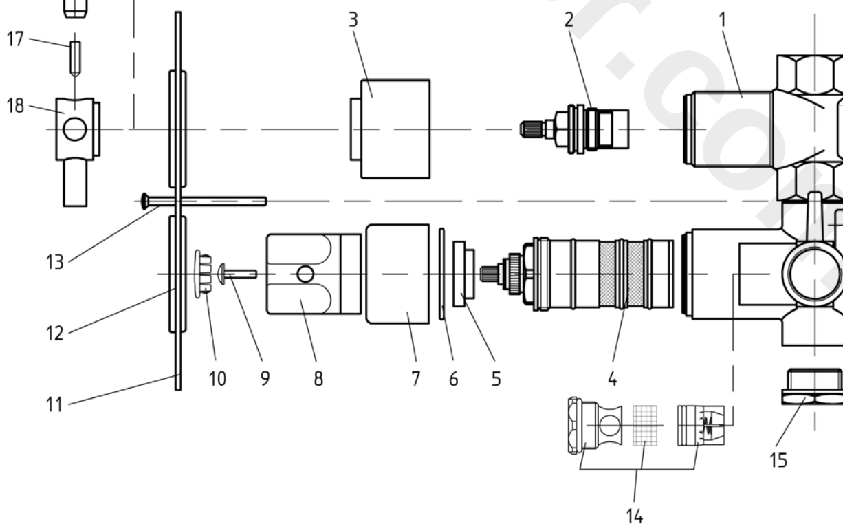
Cruzeta Cross handle
