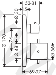
AXOR Starck 10720000
