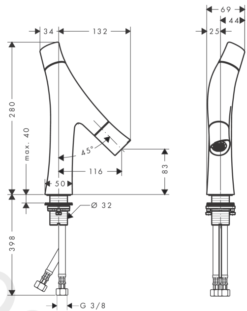
Scale drawing
