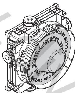
1967.045 2 Outlet First Fix Assembly
