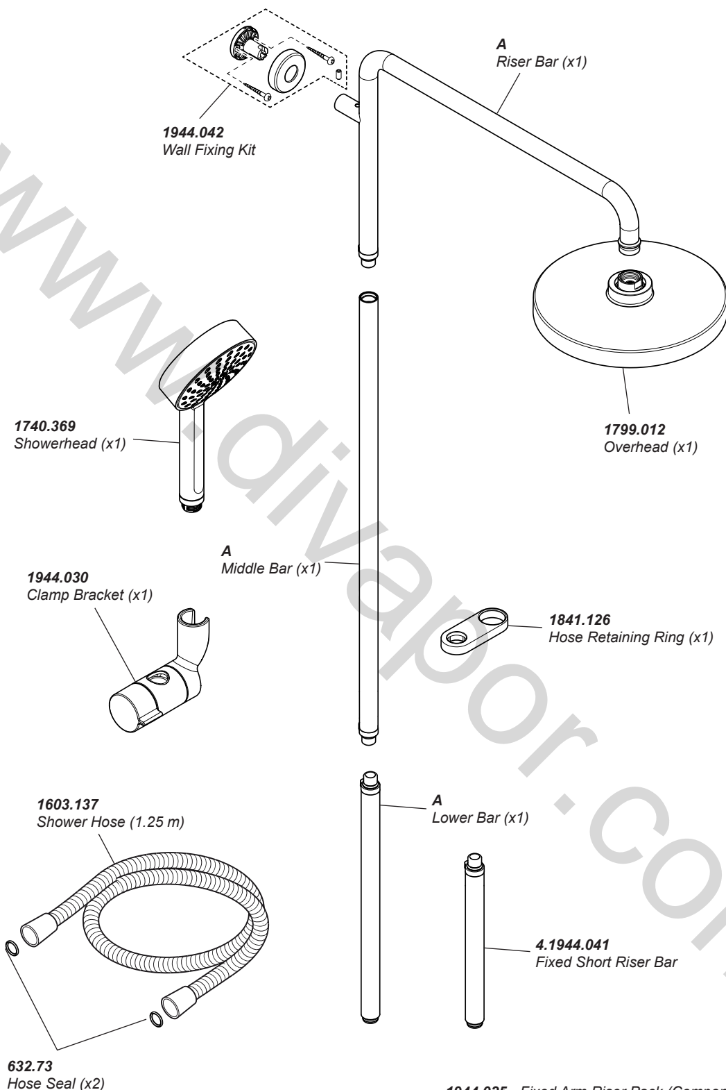
1944.025 Fixed Arm Riser Pack (Components marked as 'A')
