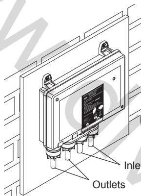
Mounting on a Vertical Surface
