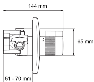
BIR+ deluge head
