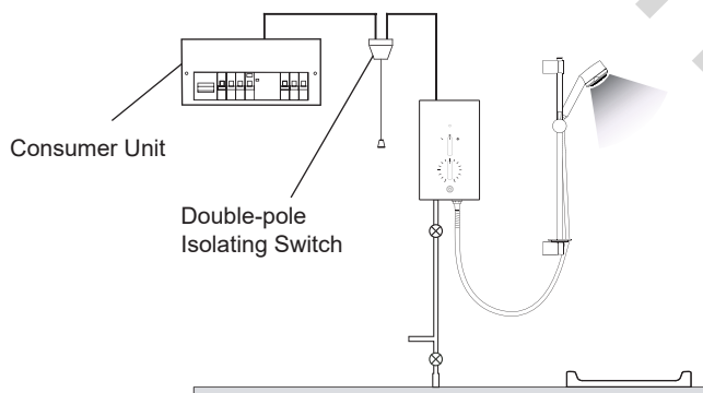
Plumbing and Electrical Schematic
